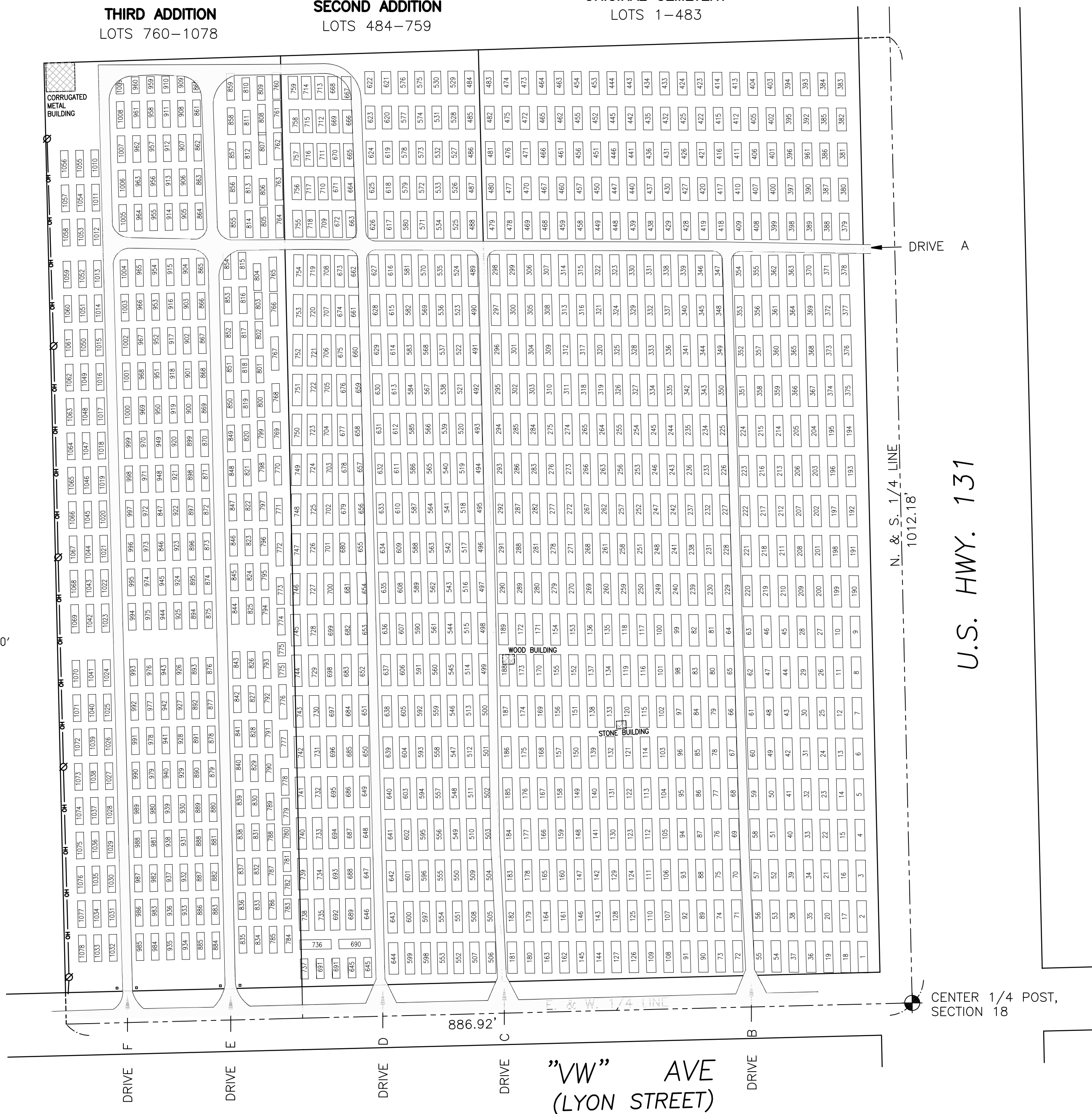
TYPICAL LOT LAYOUT FOR THIRD ADDITION (UNLESS SHOWN OTHERWISE)
