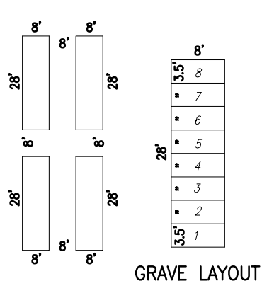
TYPICAL LOT LAYOUT FOR THIRD ADDITION (UNLESS SHOWN OTHERWISE)
